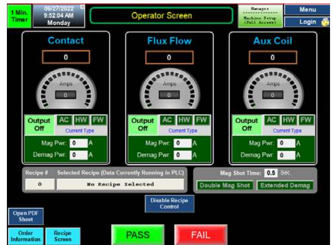
Ability to run in recipe mode (automatically loads correct test parameters) or manual mode (allows user the ability to control outputs, waveforms, and current settings) MD3-2060 pictured above
